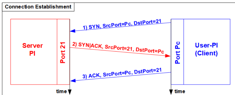
Figure 1-2 Connection Establishment on Control port
