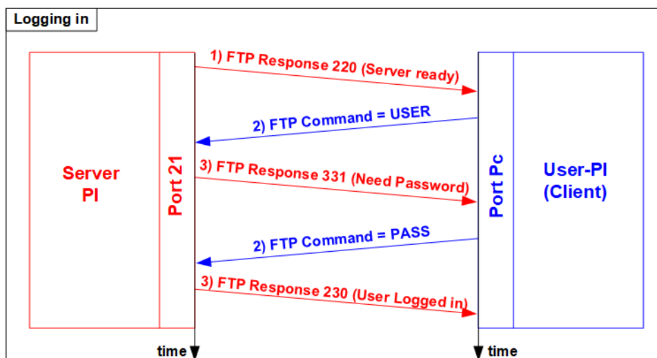
Figure 1-3 User Authentication
