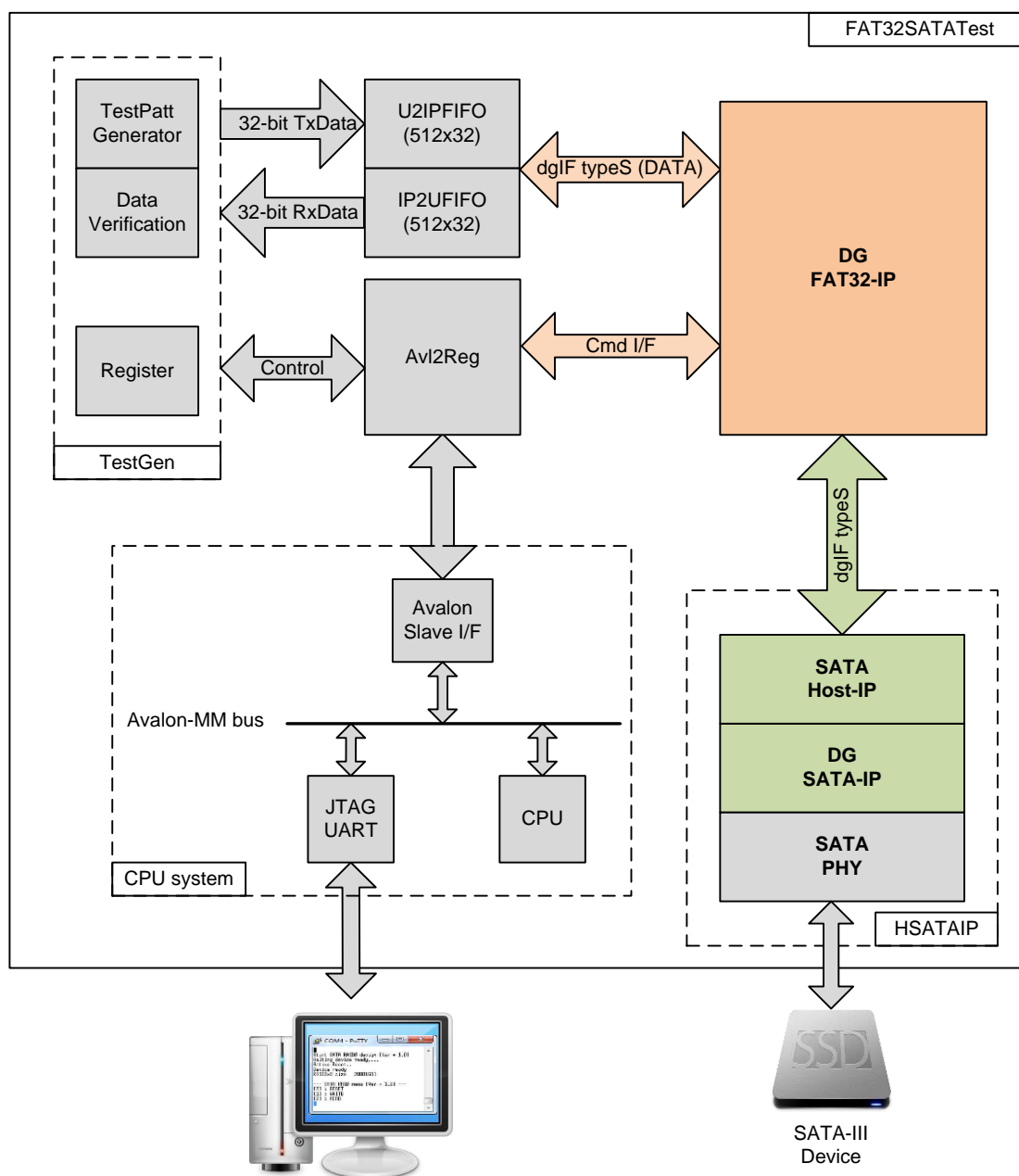
Figure 2-1 FAT32-IP for SATA Demo System
