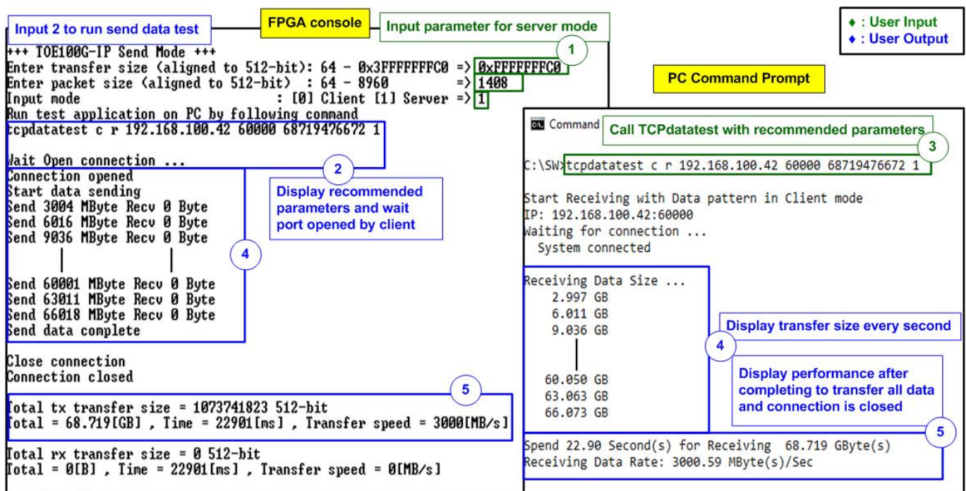
Figure 3-4 Send data test by using non-jumbo frame with data verification
