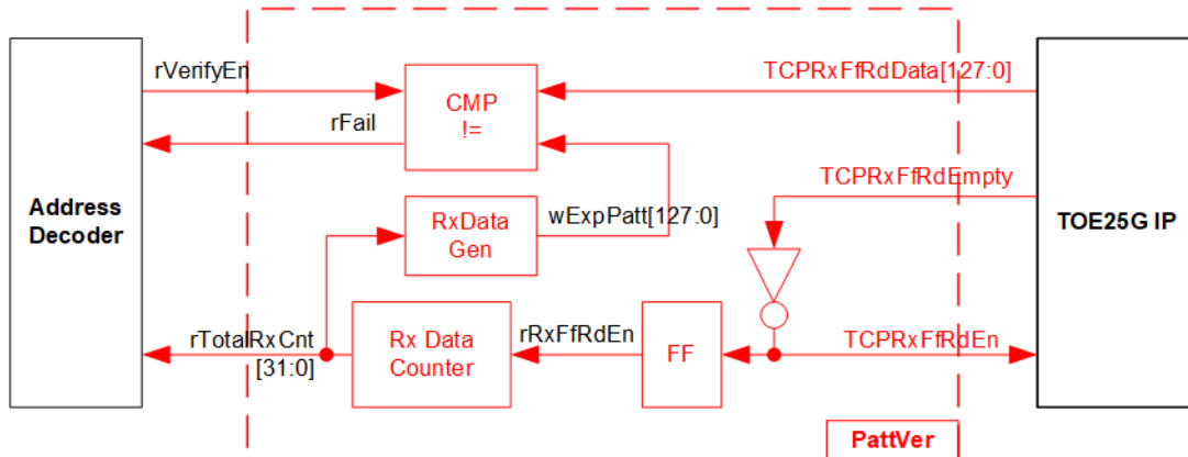
Figure 2-10 PattVer block
