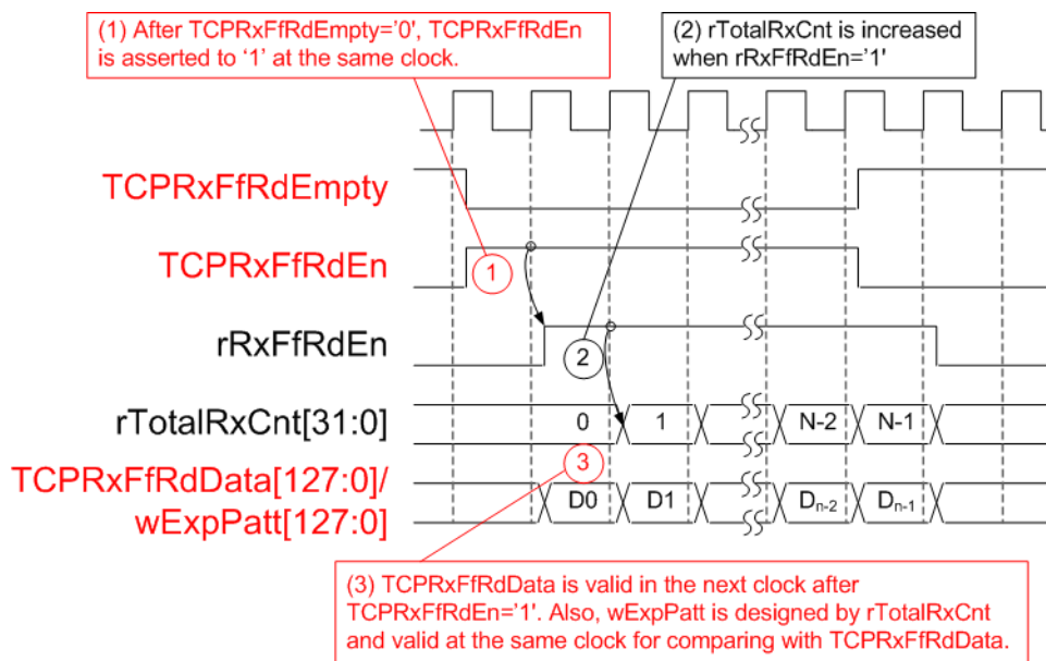
Figure 2-11 PattVer Timing diagram
