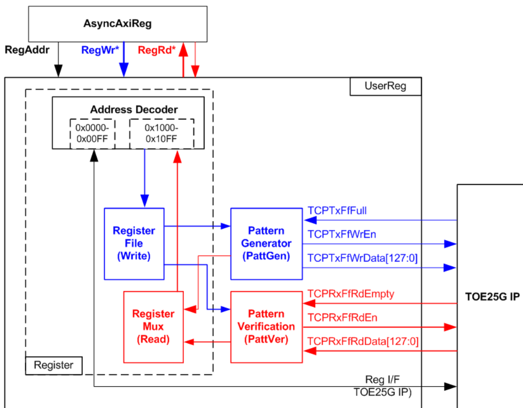
Figure 2-7 UserReg block diagram
