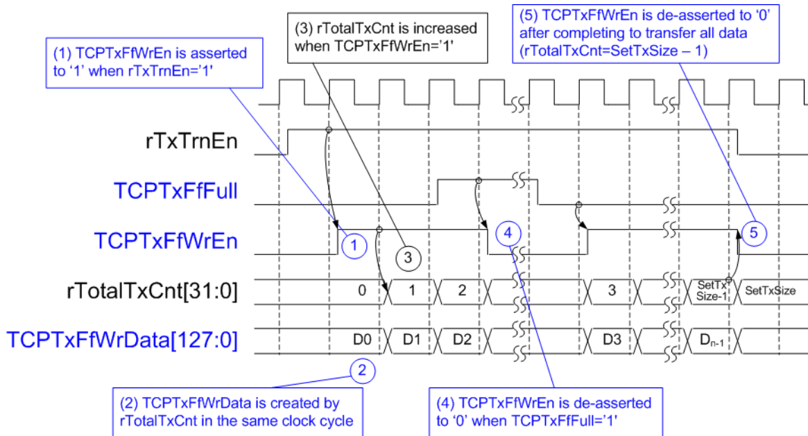
Figure 2-9 PattGen timing diagram
