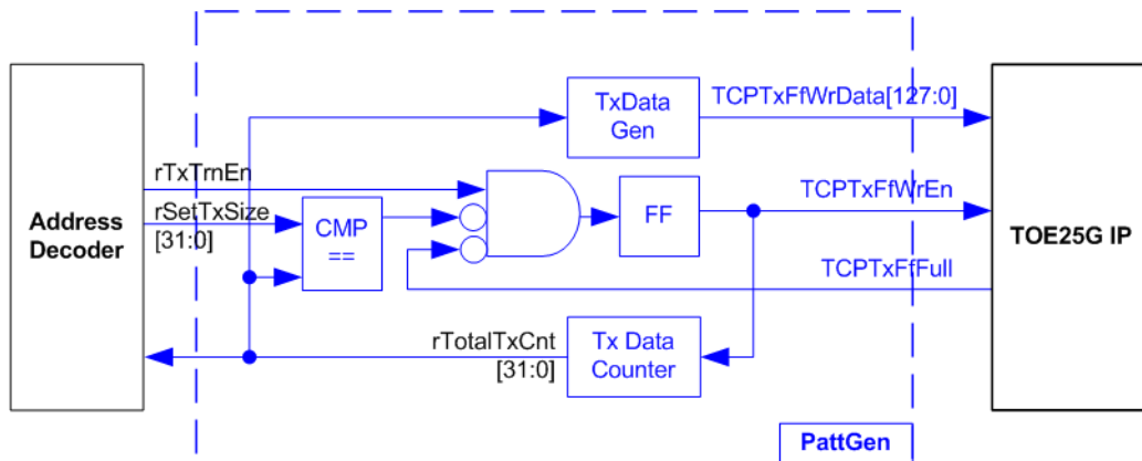
Figure 2-8 PattGen block
