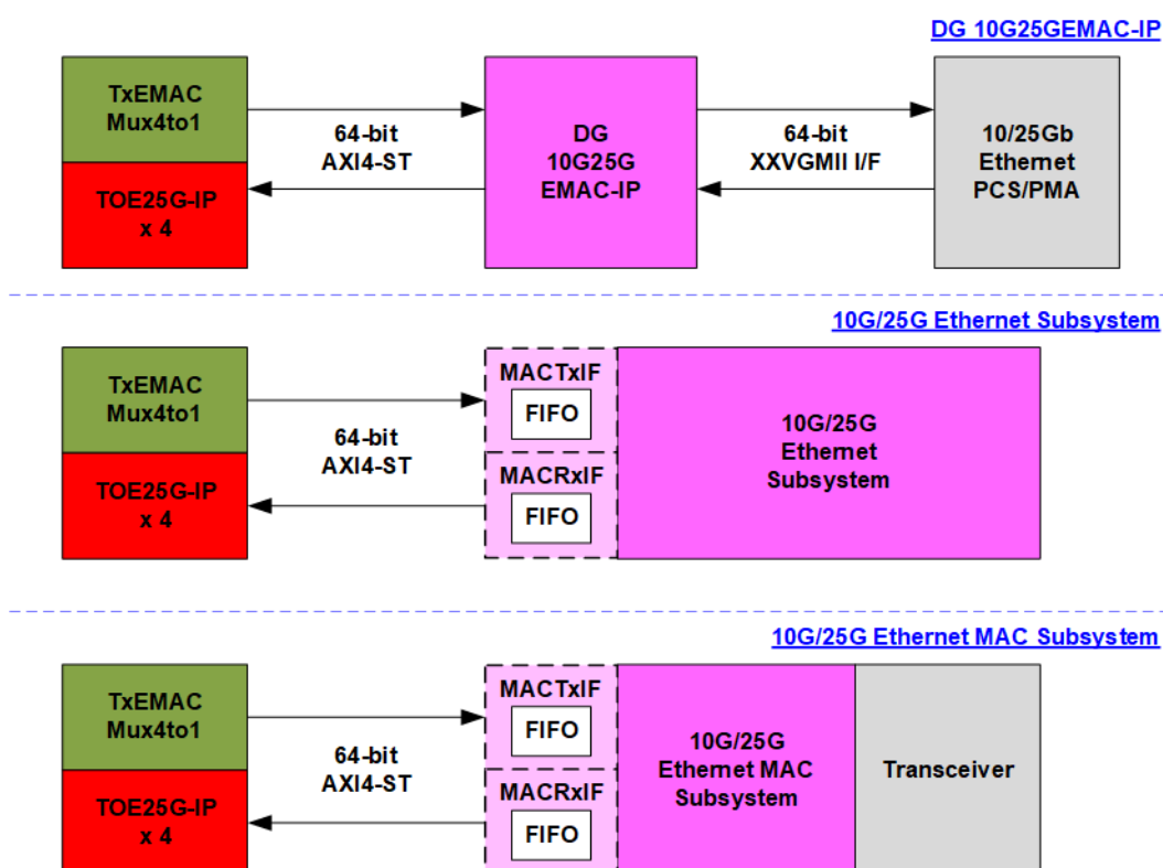
Figure 2-2 25G Ethernet System solutions for TOE25G-IP
