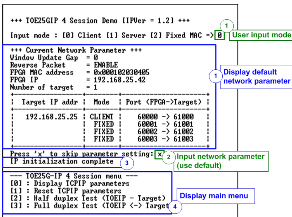
Figure 3-2 System initialization in Client mode by using default parameters
