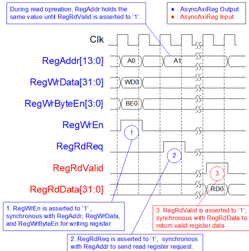
Figure 2-6 Register interface timing diagram
