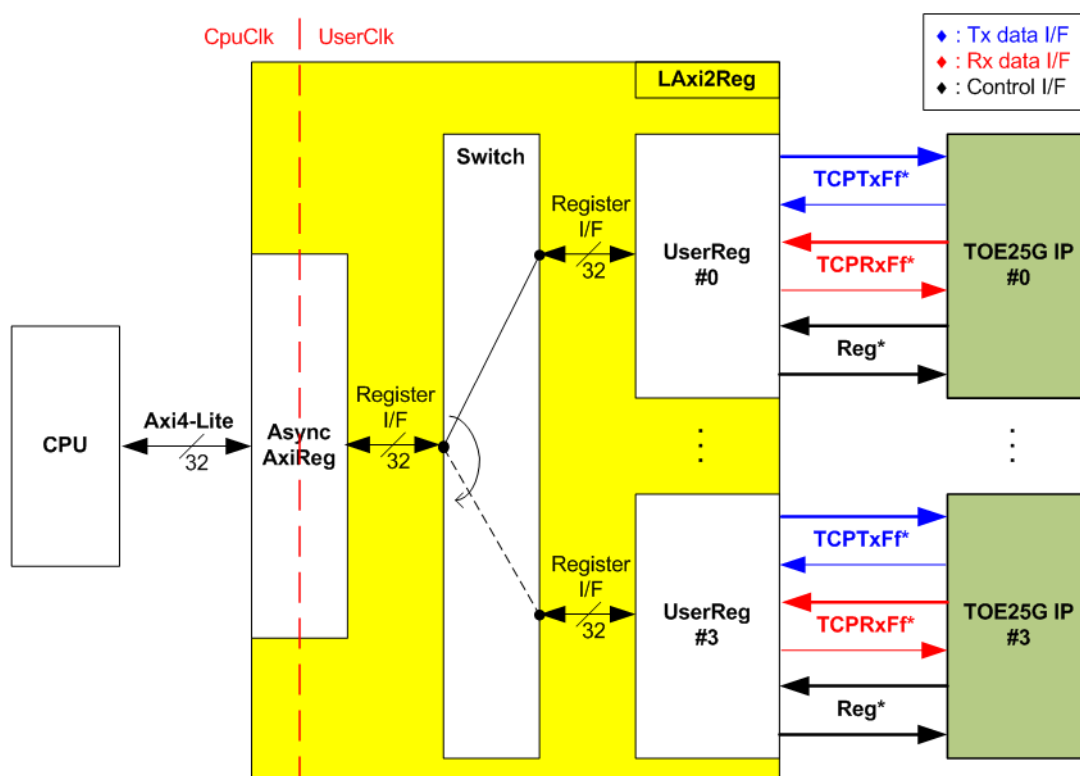
Figure 2-4 LAXi2Reg block diagram
