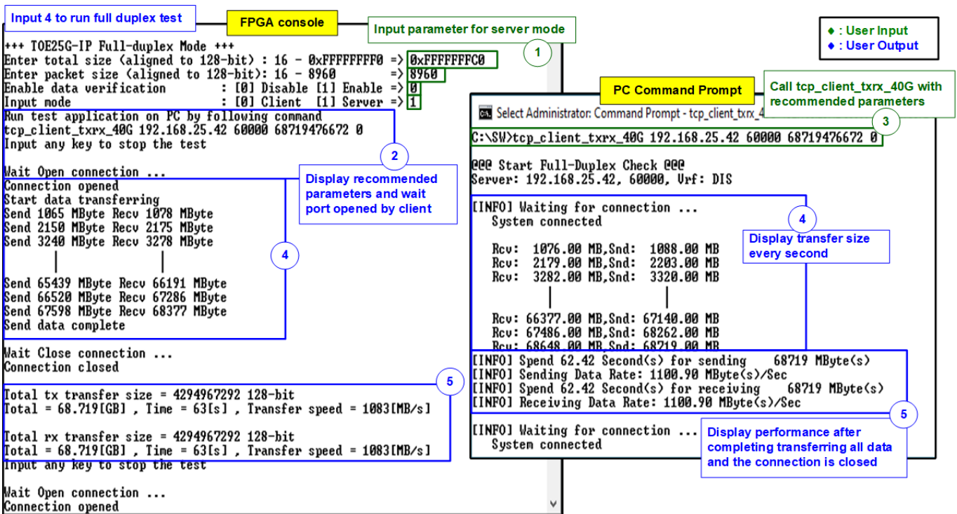
Figure 3-12 Full duplex test without data verification
