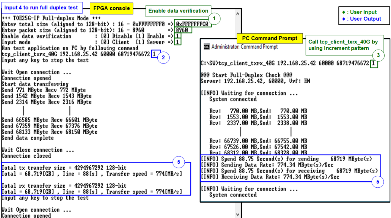
Figure 3-13 Full duplex test with data verification
