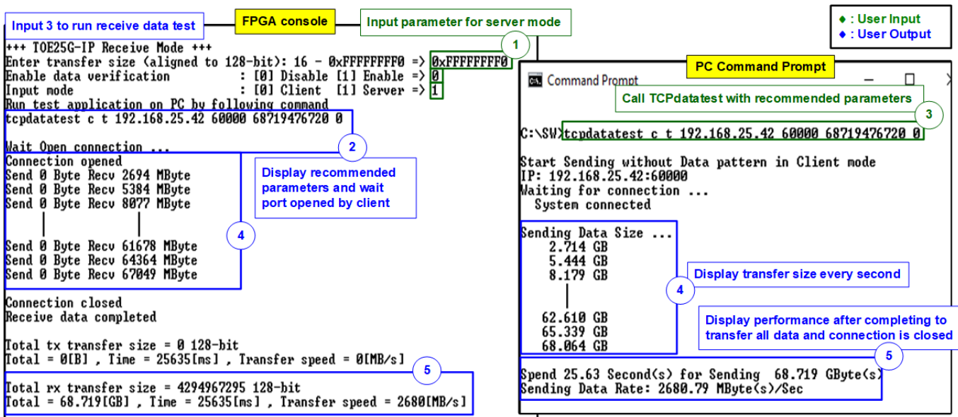
Figure 3-9 Receive data test without data verification
