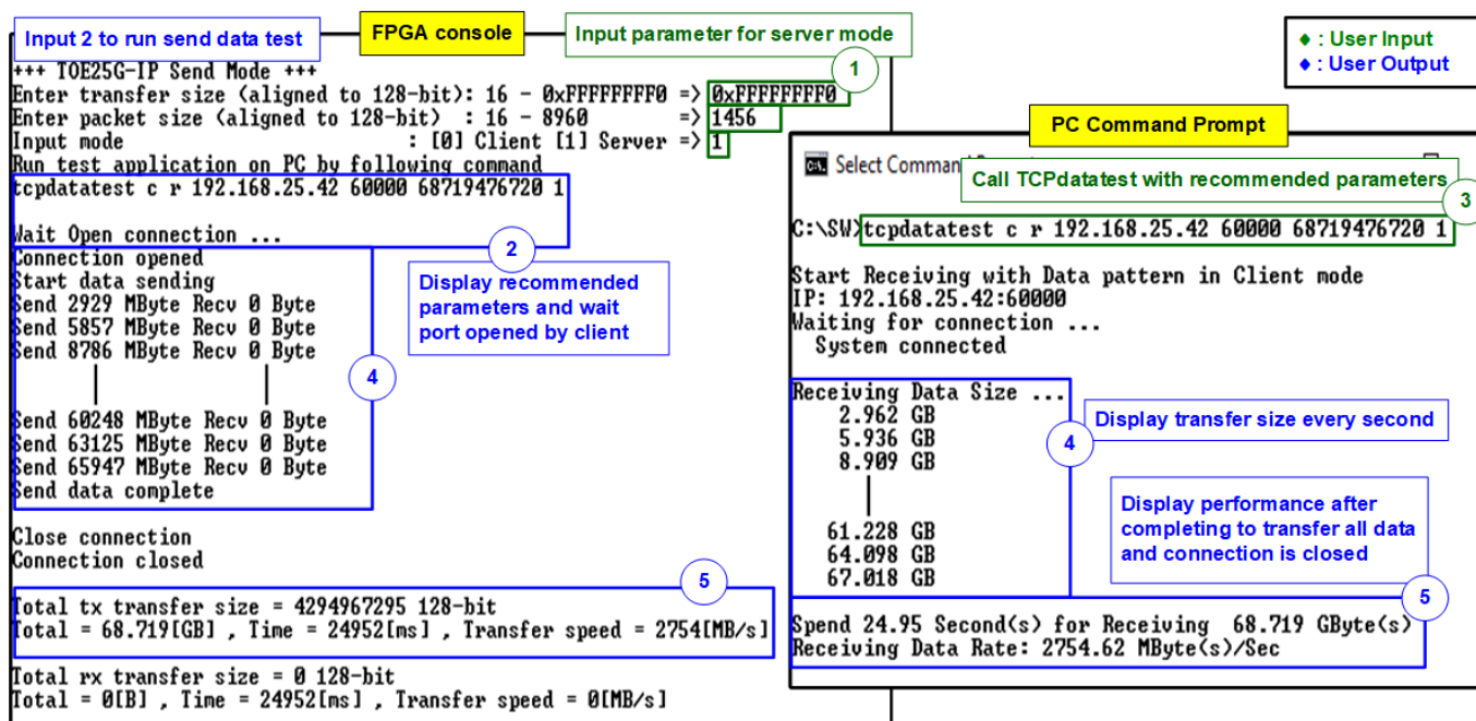
Figure 3-4 Send data test by using non-jumbo frame
