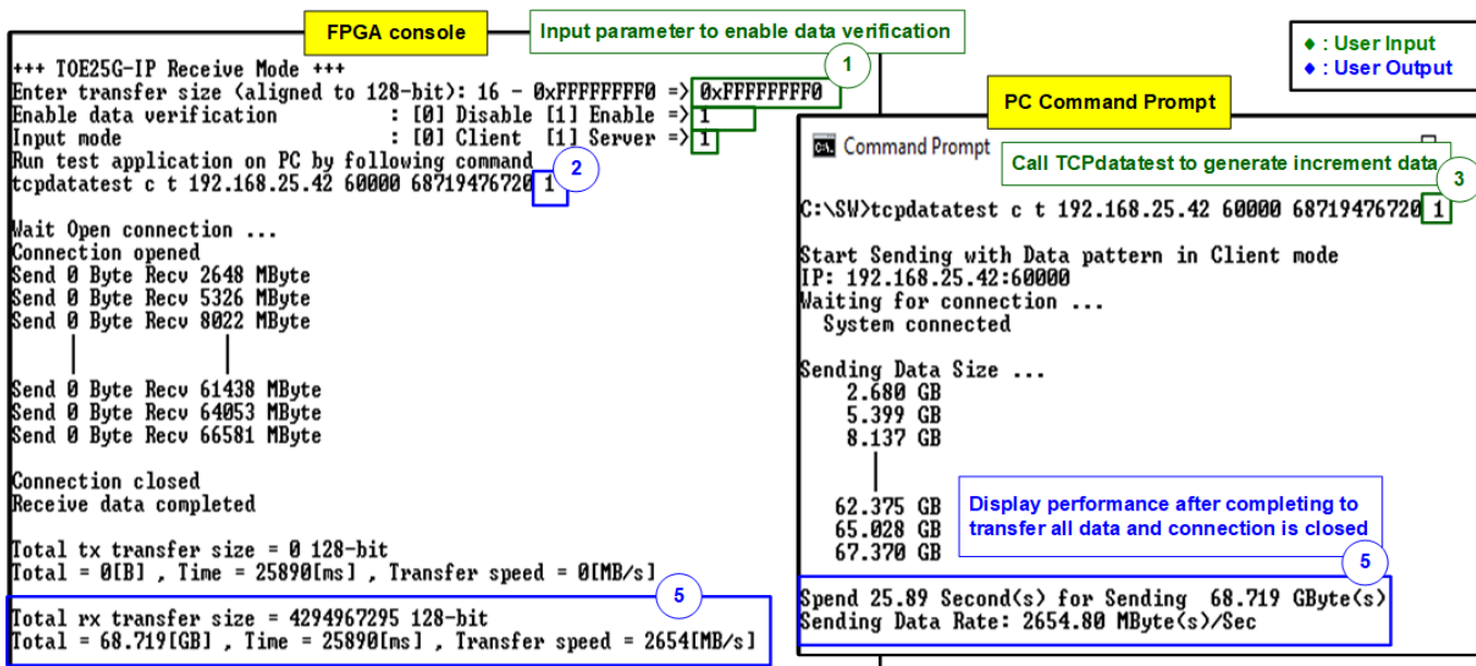
Figure 3-10 Receive data test when enabling data verification
