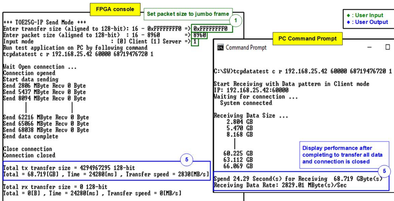
Figure 3-5 Send data test by using jumbo frame
