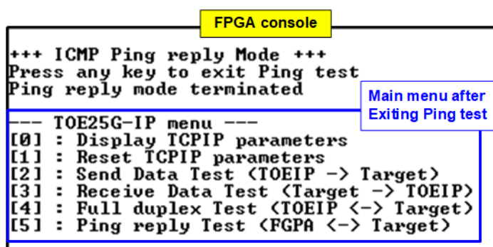
Figure 3-16 Main menu is displayed after exit the Ping test
