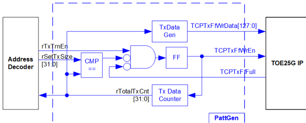
Figure 2-17 PattGen block
