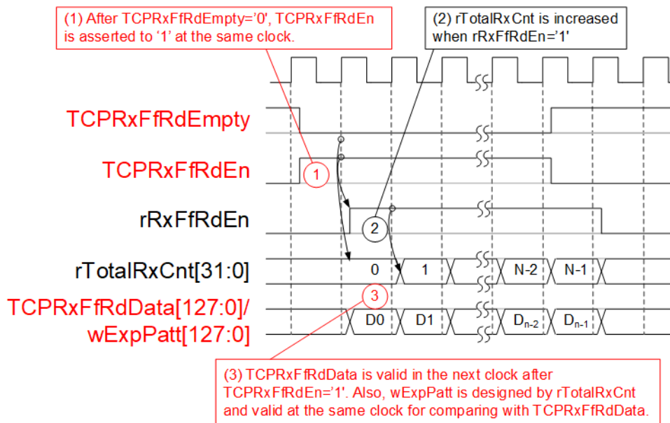
Figure 2-20 PattVer Timing diagram
