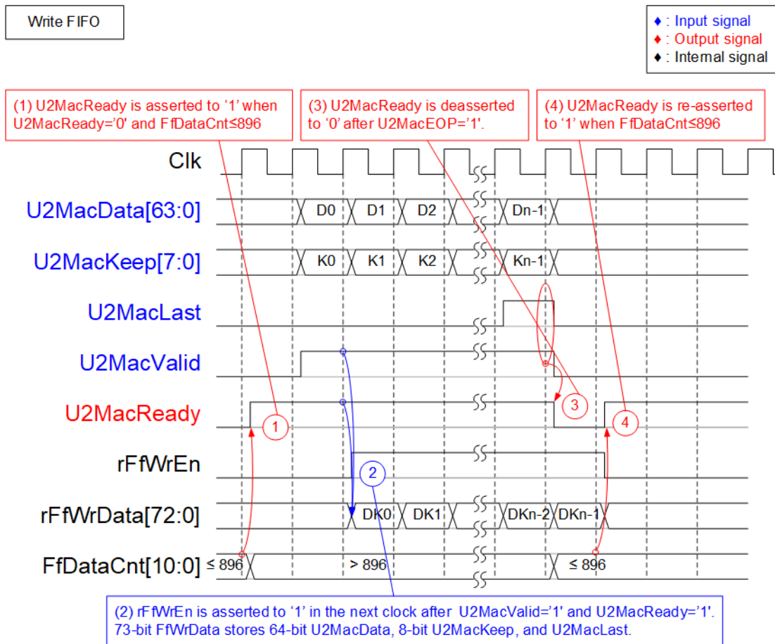
Figure 2-4 Timing diagram for transferring data from TxEMacMux2to1 to FIFO
