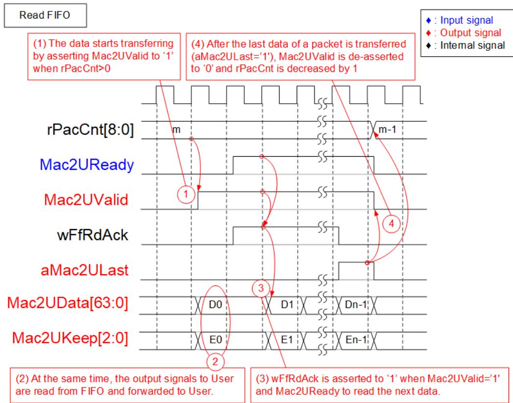
Figure 2-8 Timing diagram of data transferring from FIFO to TOE25G-IP
