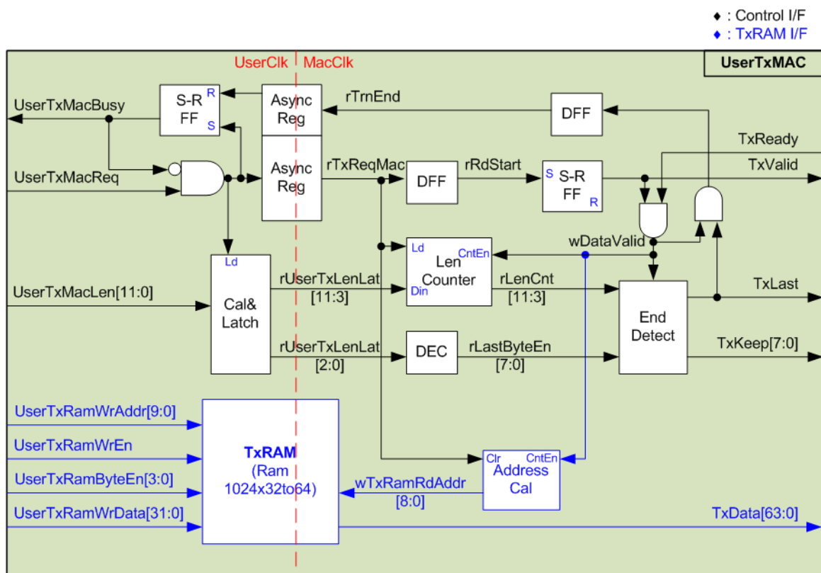
Figure 2-11 UserTxMAC Logic Diagram
