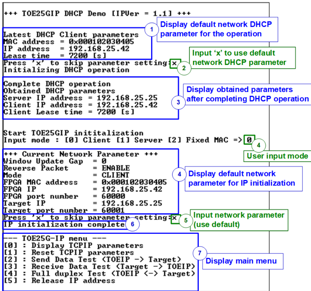
Figure 4-1 Boot menu of DHCP demo
