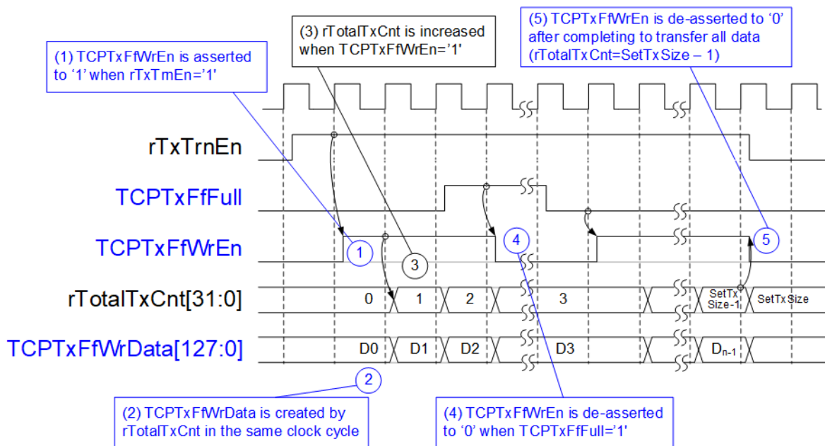
Figure 2-18 PattGen timing diagram
