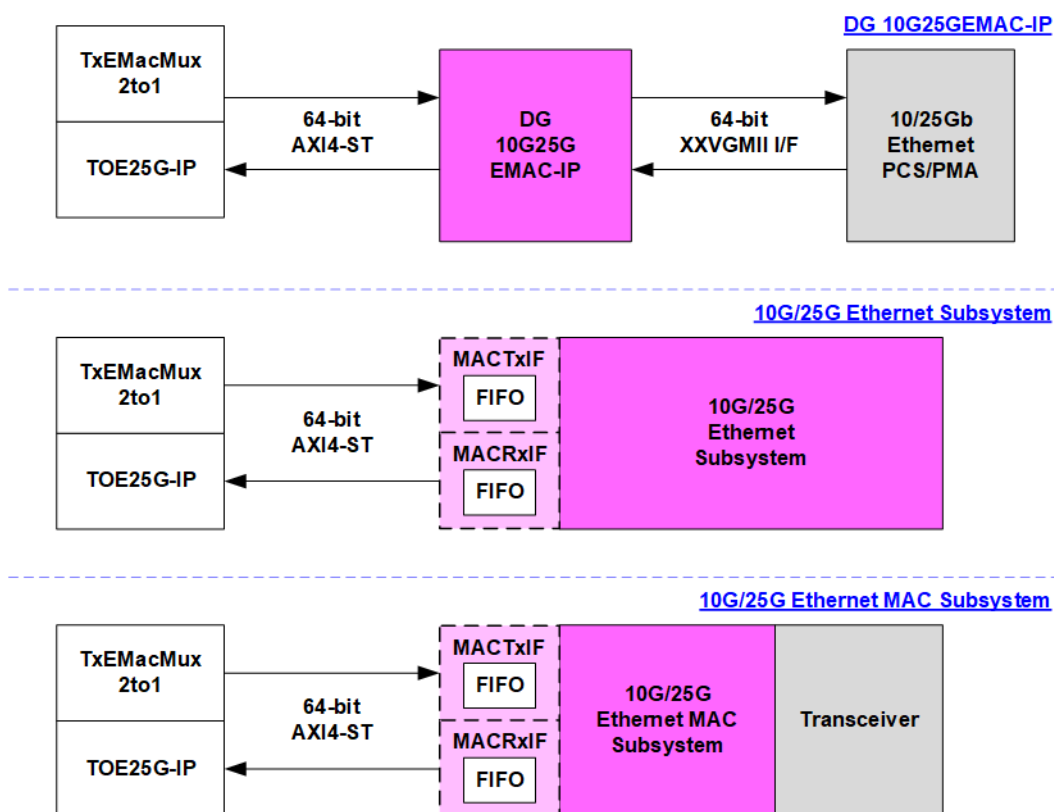
Figure 2-2 TOE25G-IP with several Ethernet system solutions
