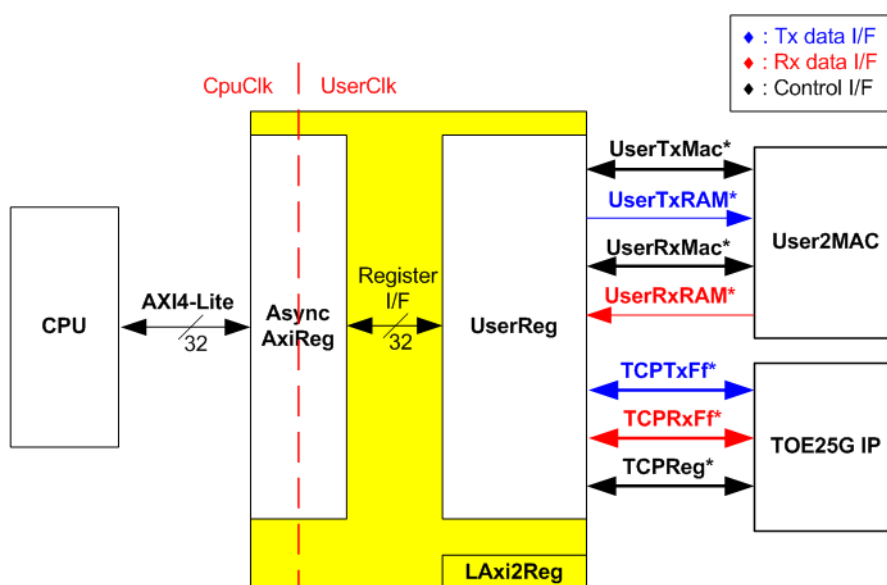
Figure 2-13 LAXi2Reg block diagram
