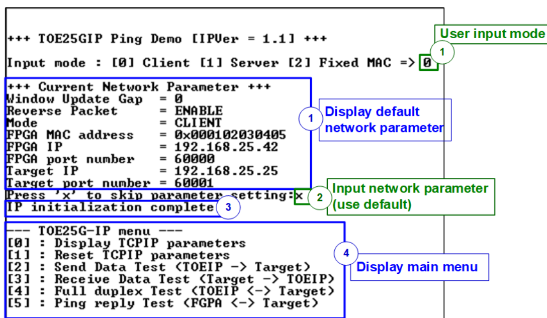
Figure 3-1 Boot menu of Ping demo
