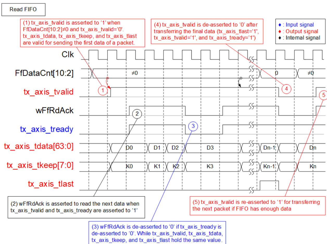
Figure 2-5 Timing diagram of data transferring from FIFO to EMAC
