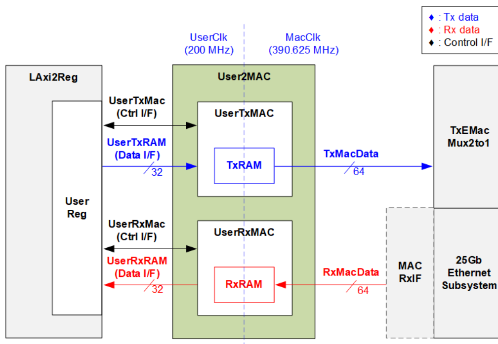
Figure 2-10 User2MAC block diagram
