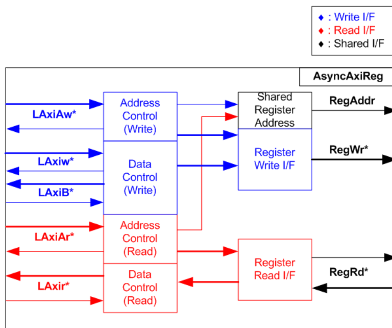
Figure 2-14 AsyncAxiReg interface
