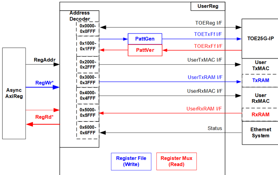
Figure 2-16 UserReg block diagram
