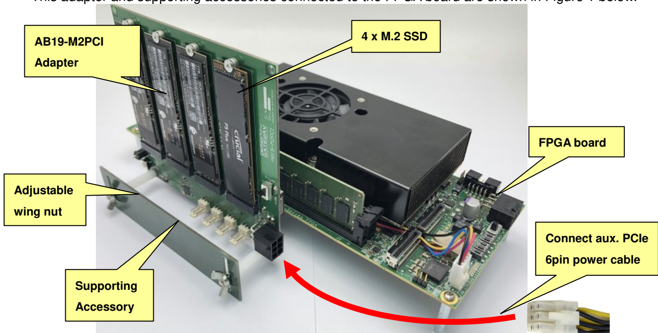
Figure-1: AB19-M2PCIe adapter with supporting accessory
