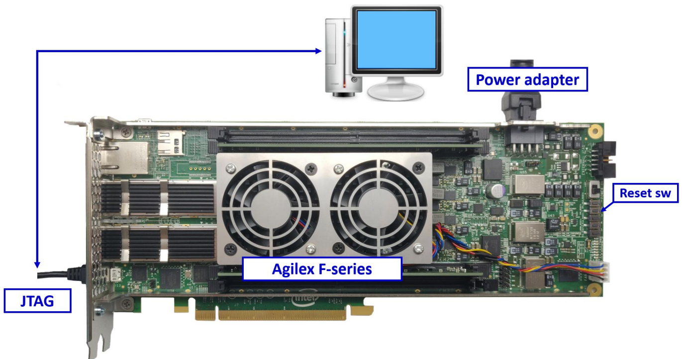
Figure 1-1 AES256GCM100GIP demo environment on Agilex F-series board
