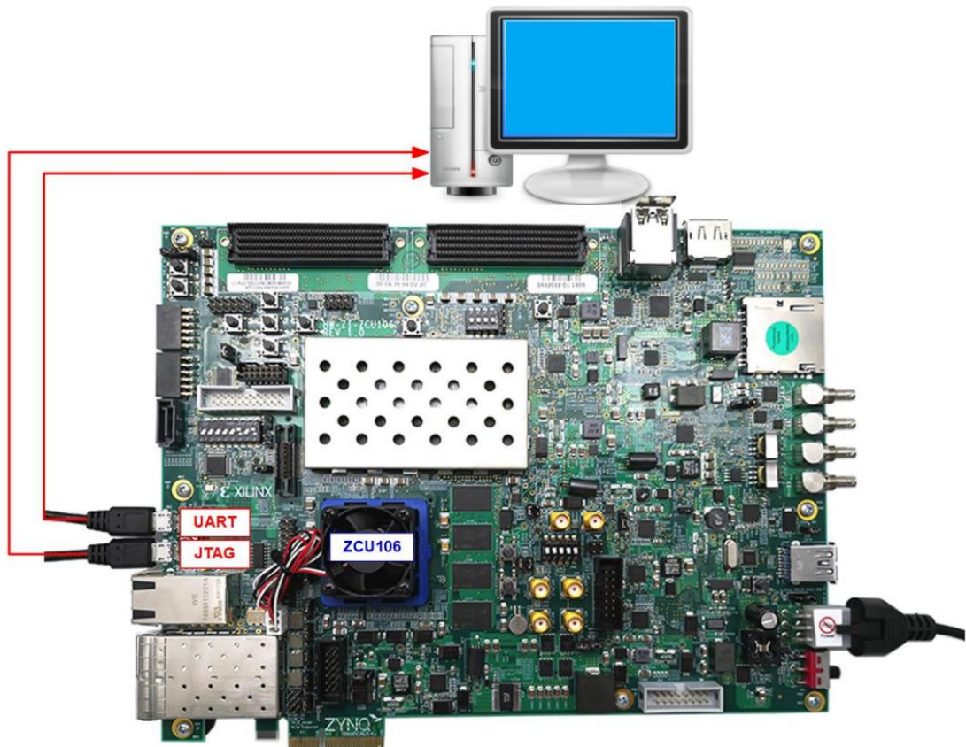
Figure 1-1 AES256GCM10G25GIP demo environment on ZCU106 board
