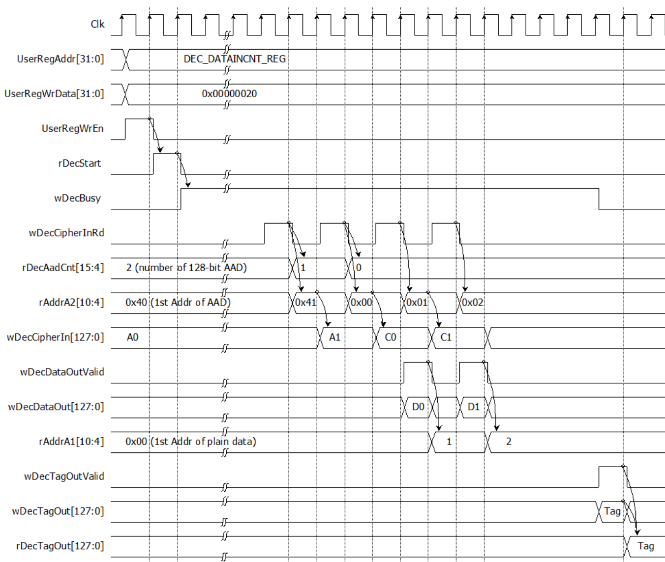
Figure 2-6 Timing diagram of decryption process
