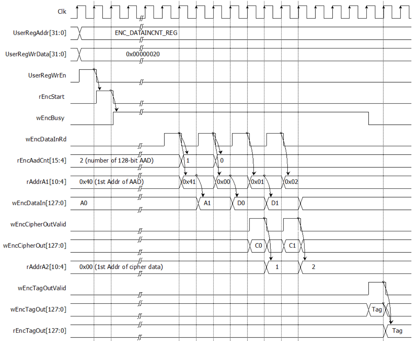
Figure 2-5 Timing diagram of encryption process
