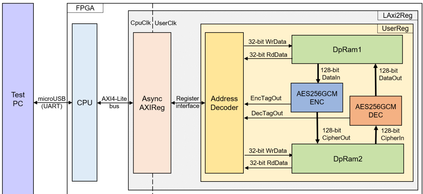
Figure 2-1 AES256GCM10GIP reference design block diagram
