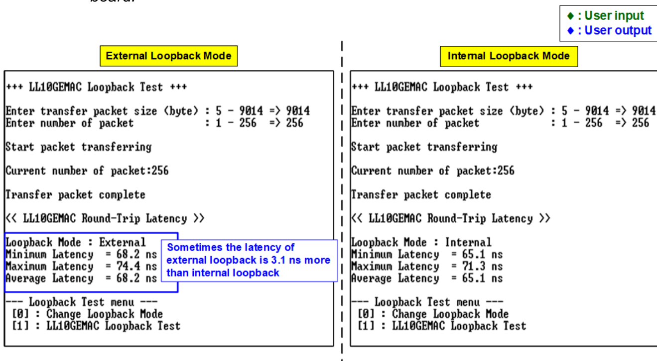
Figure 1-3 Different latency time found when running internal and external loopback
