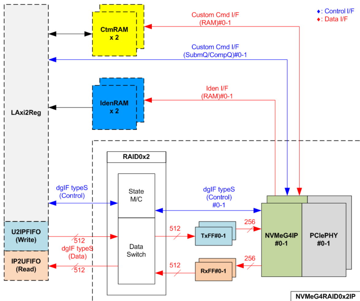
Figure 2-7 NVMeG4RAID0x2 hardware
