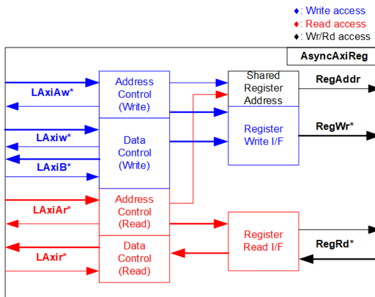
Figure 2-13 AsyncAxiReg Interface
