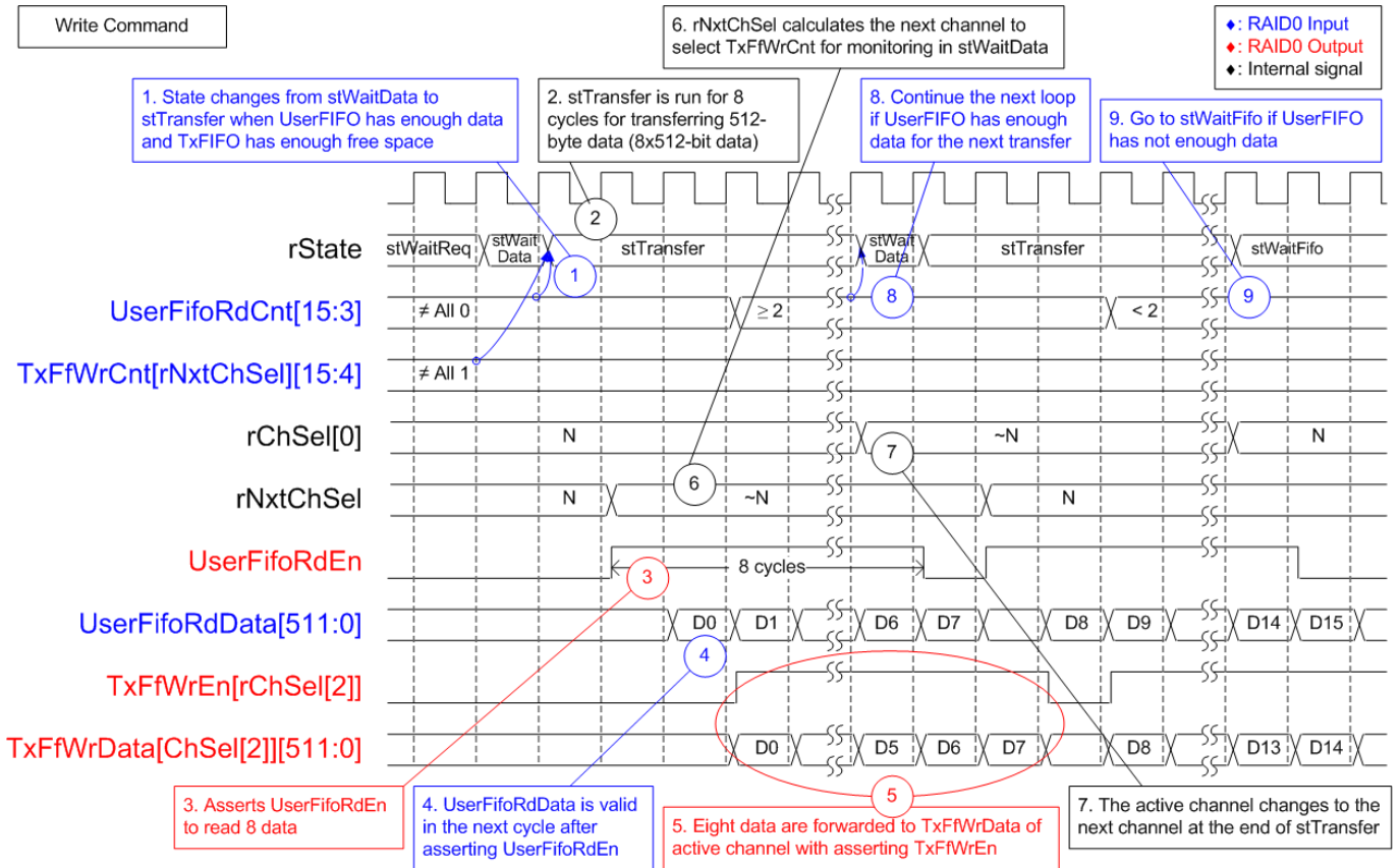
Figure 2-10 Raid0x2 timing diagram in Write command
