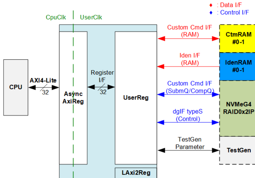
Figure 2-12 CPU and peripherals hardware
