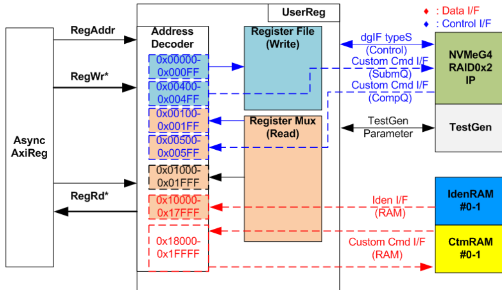
Figure 2-15 UserReg Interface
