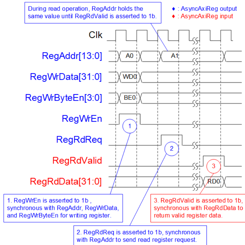
Figure 2-14 Register interface timing diagram
