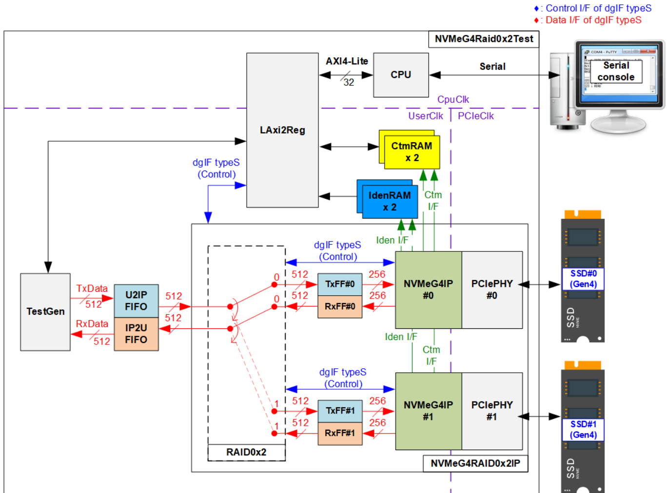
Figure 2-1 RAID0x2 demo system using NVMeG4-IP
