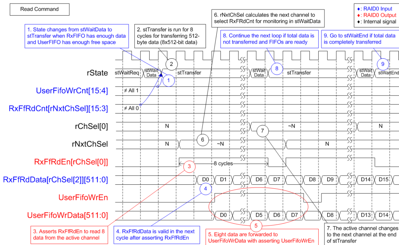
Figure 2-11 Raid0x2 timing diagram in Read command
