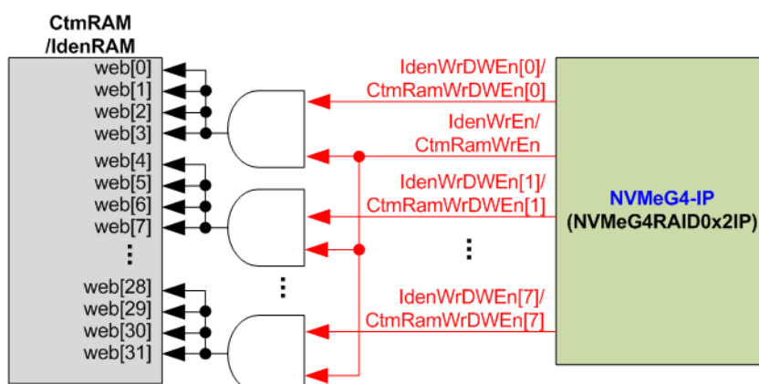
Figure 2-8 Byte write enable conversion logic
