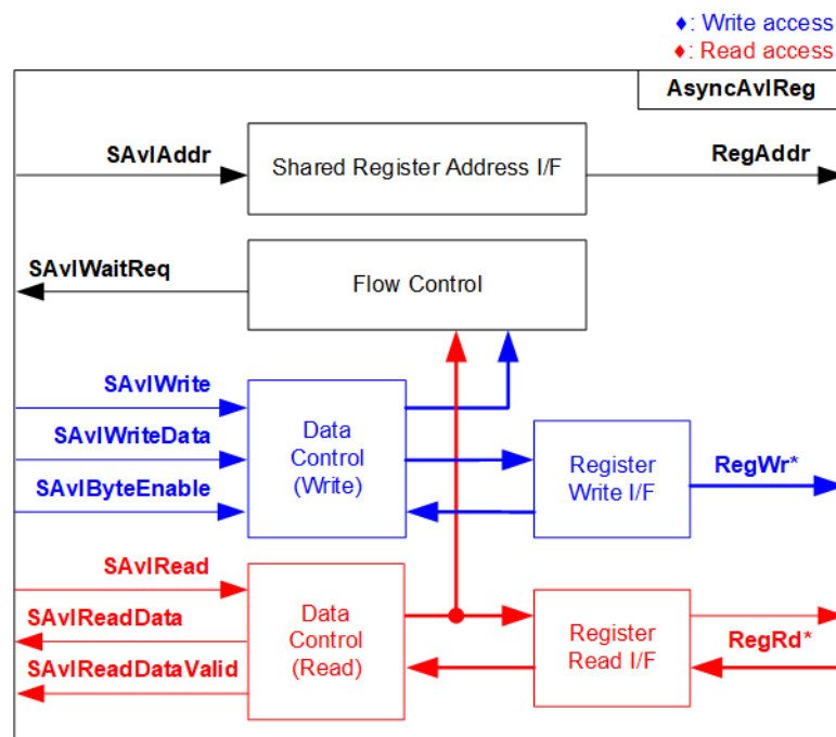
Figure 2-10 AsyncAvlReg Interface
