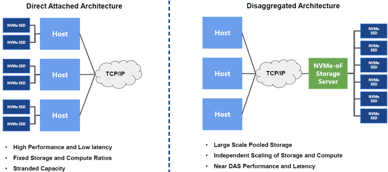
Figure 1-1 NVMe/TCP usage
