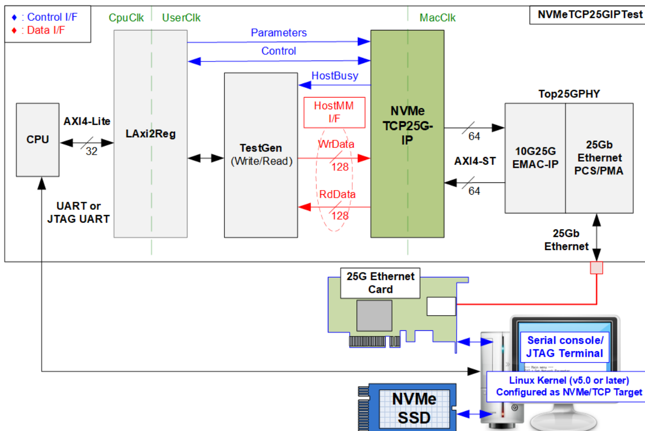
Figure 2-1 NVMeTCP25G-IP demo hardware
