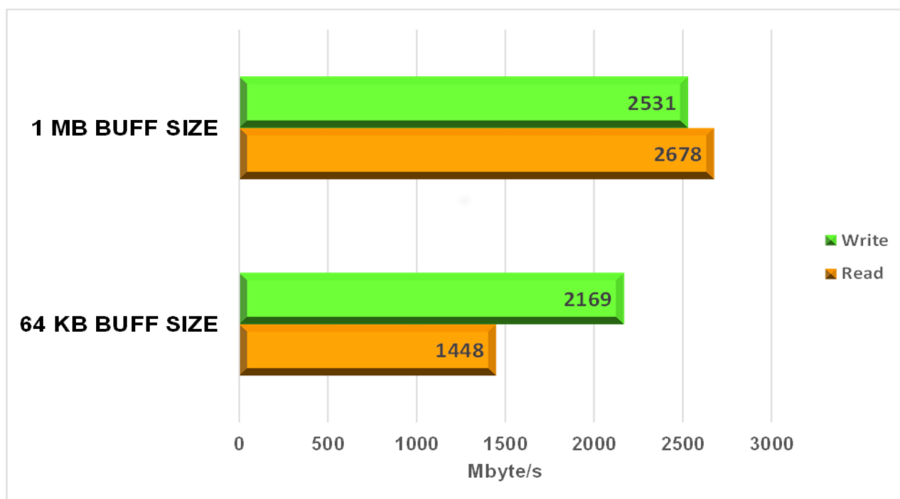
Figure 4-1 Test Performance of NVMeTCP25G-IP demo
