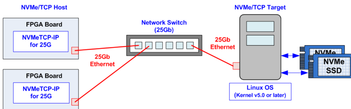
Figure 1-5 NVMe/TCP system by using NVMeTCP25-IP
