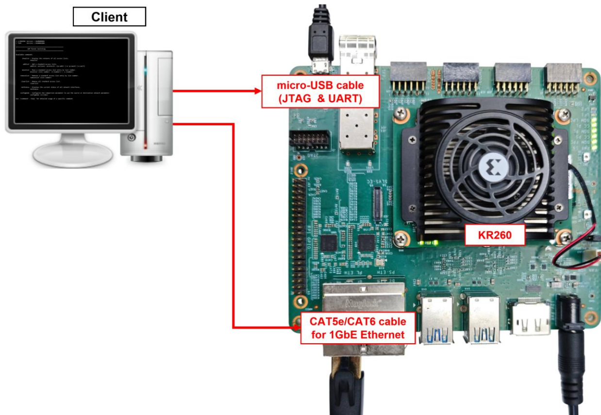
Figure 1 QUIC1GCIP demo environment on KR260 board
