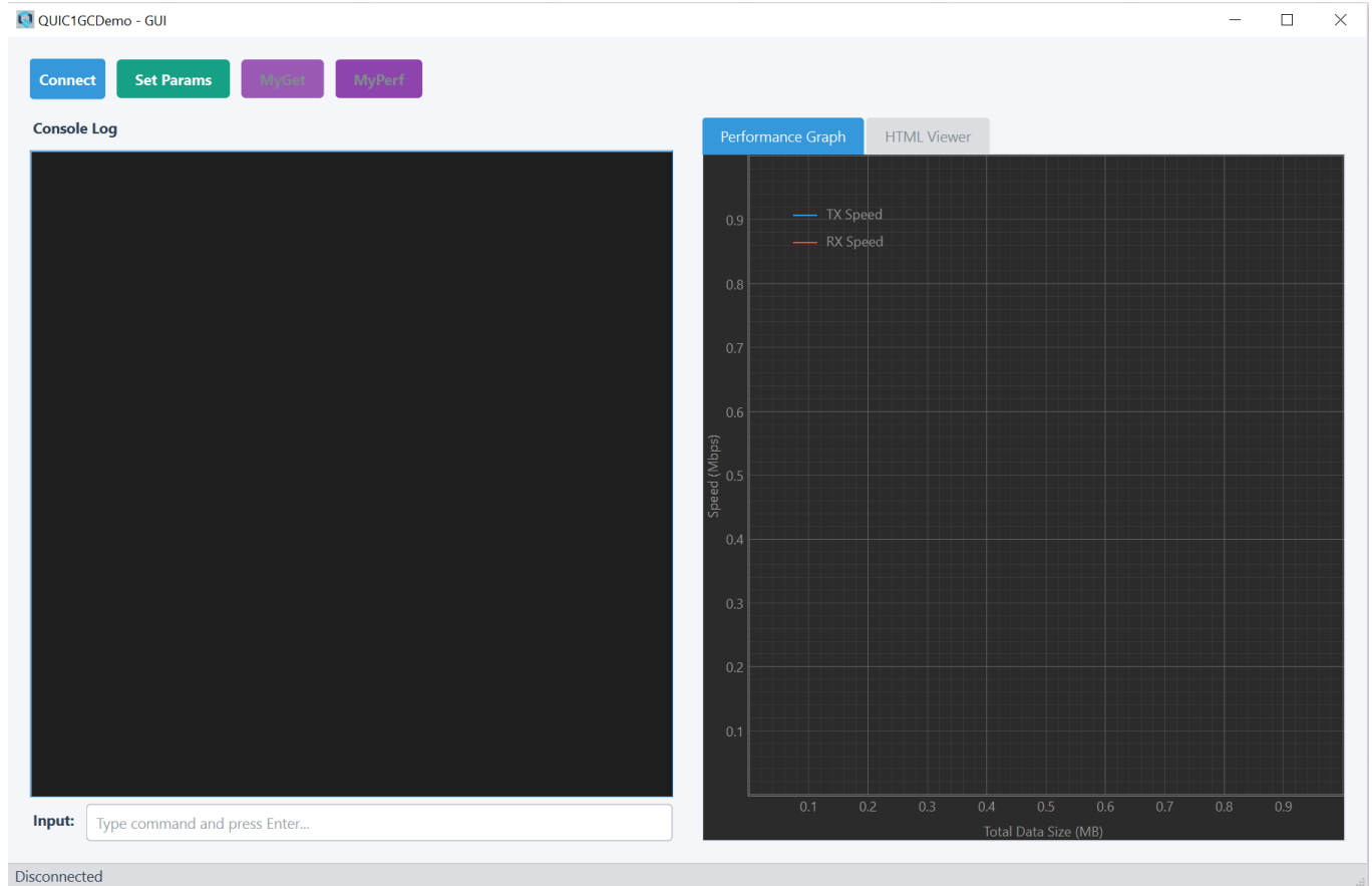
Figure 33 QUIC1GCDemo-GUI window
