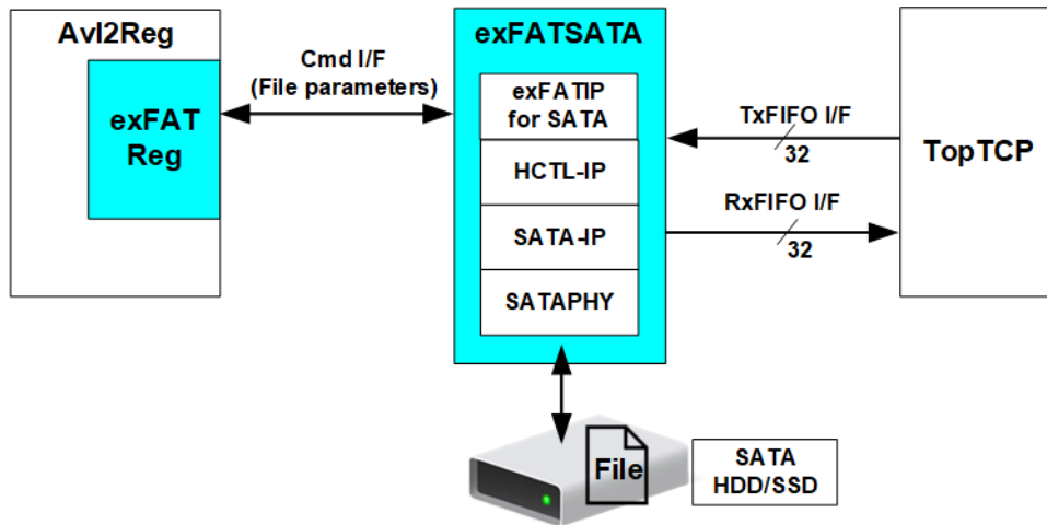
Figure 2-12 exFATSATA Block Diagram
