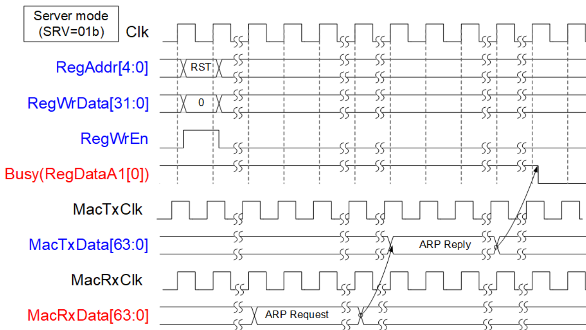
Figure 4: IP Initialization in Server mode
