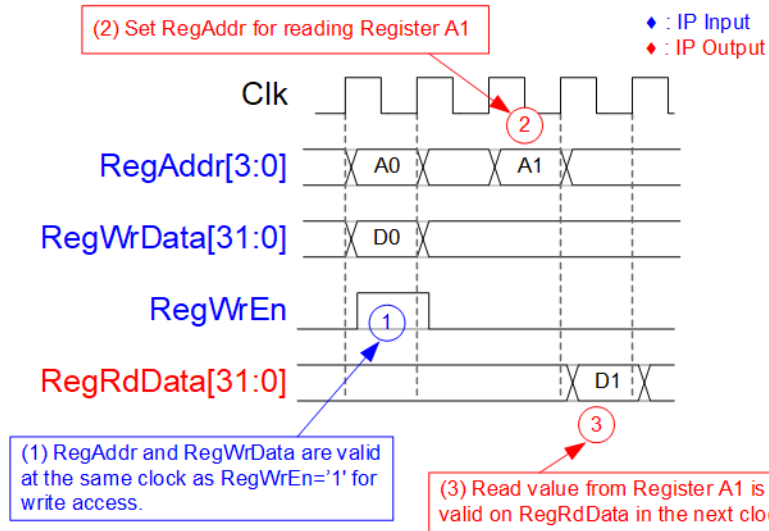
Figure 6: Register interface timing diagram
