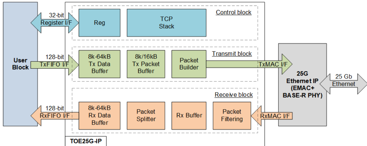
Figure 2: TOE25G IP Block Diagram
