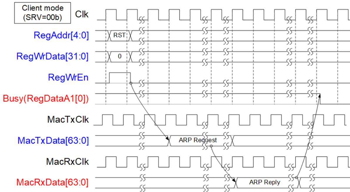
Figure 3: IP Initialization in Client mode
