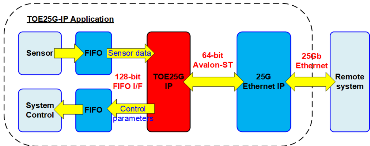
Figure 1: TOE25G IP Application
