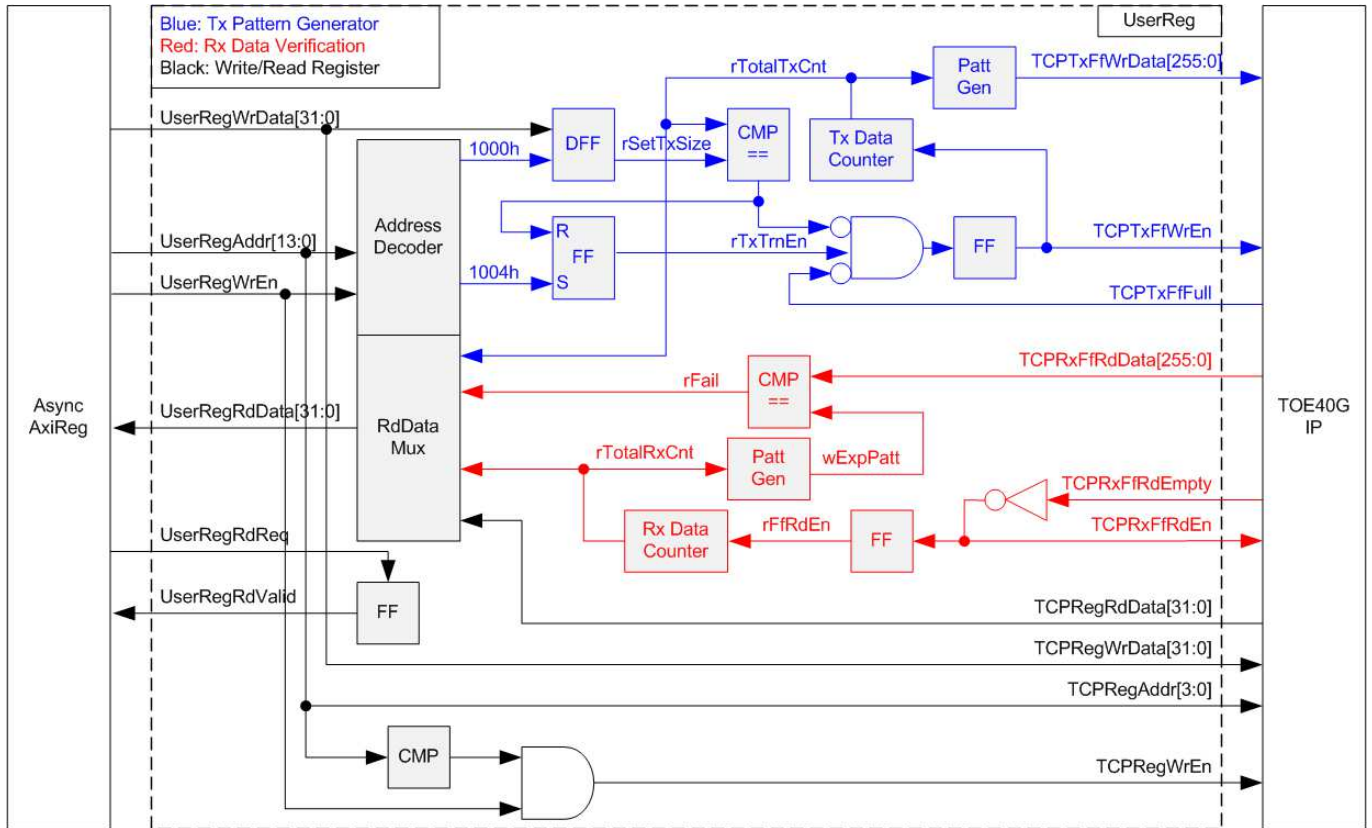
Figure 2-8 UserReg block diagram
